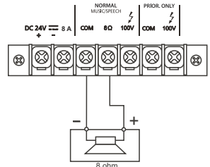
Connecting a single speaker to 8 ohm output
